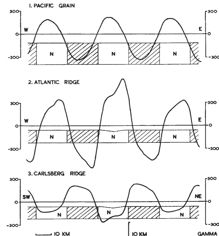
Fig. 4. Magnetic profiles computed for various crustal models. Crustal blocks marked N, normally magnetized; diagonally shaded blocks, reversely magnetized. Effective susceptibility of blocks, 0.0027, except for the block under the median valley in profiles 2 and 3, 0.0053.
