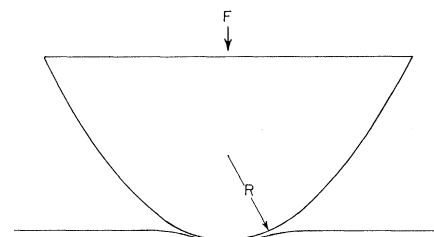
Fig. 1. Diagram of a spherically tipped diamond indentor of radius R pressed against an initially flat diamond anvil with a force F . Typically the indentor is a single crystal diamond 1/500 to 1/1000 carat with a tip radius of 2 to 20 \mu\text{m} , and it is mounted in a steel shank. The flat is single crystal diamond (about \frac{1}{2} carat) with parallel faces, also mounted in a steel shank. Because of the small size of the indentor, the damage to the flat is quite local and many tests can be made on the same flat if different areas are used.
